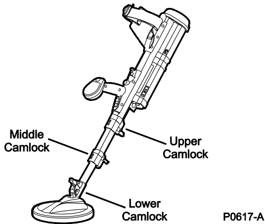
Figure 7: Camlock Locations
