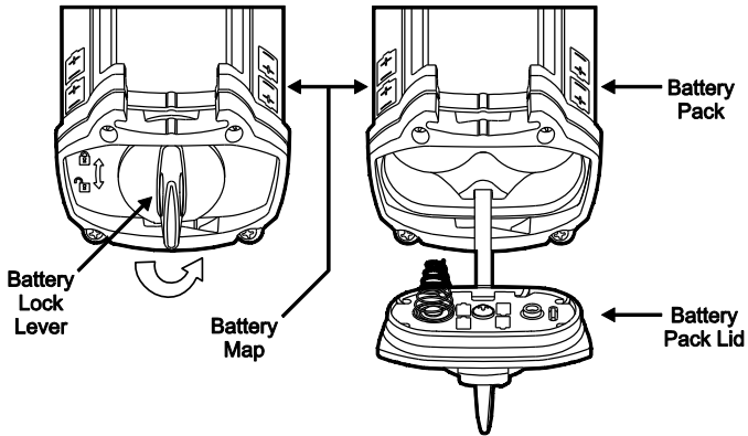
Figure 5: Removing the Battery Pack Lid
